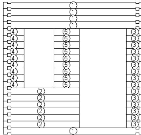
Detailed display of a wall with scarf joint
